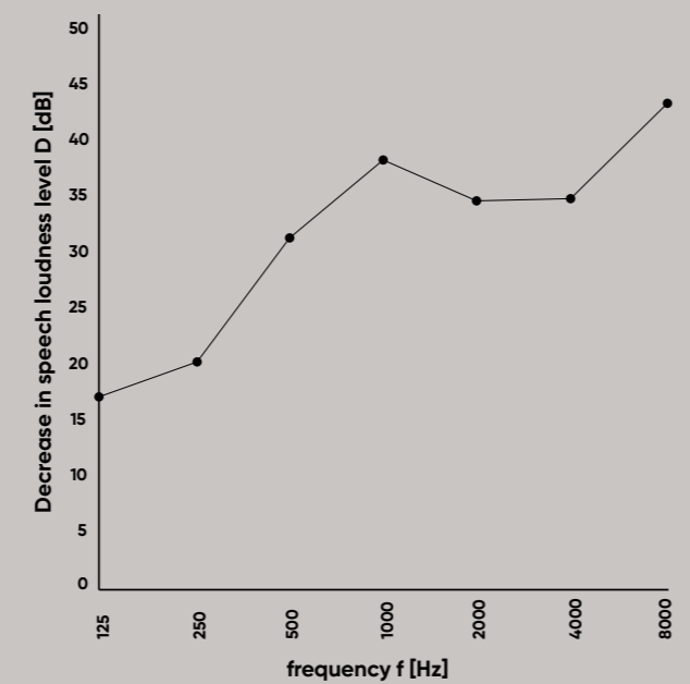
Reduction in speech loudness level
