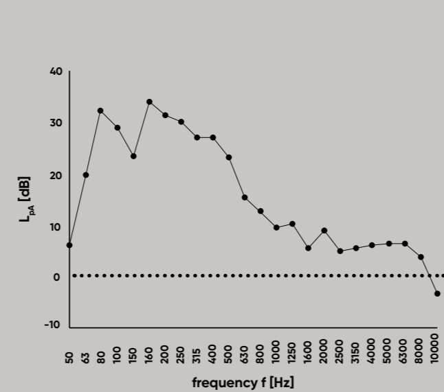
Sound level of ventilation inside the booth
