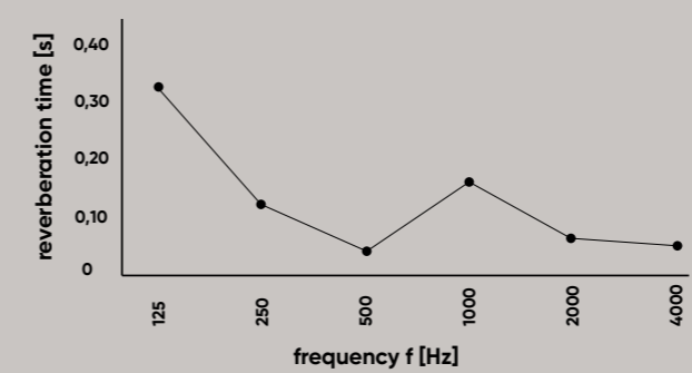
Reverberation time inside the booth
