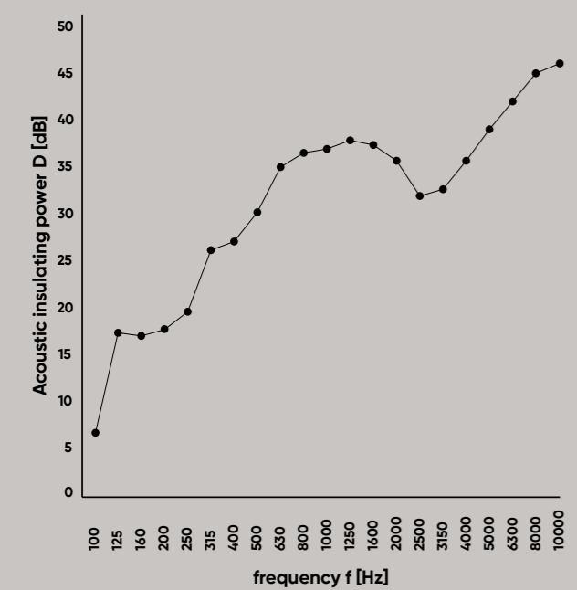
Weighted acoustic insulating power index
